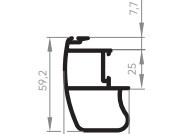
EXL-505 Montante bi-tubular central externo 0,803 Kg/m
