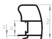
EXL-504 Montante bi-tubular central interno 0,790 Kg/m
