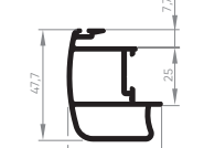
EXL-350 Montante bi-tubular central externo 0,714 Kg/m
