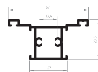
EXL-086 Travessa vertical com alhal maxim-ar 0,574 Kg/m
