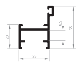
EXL-079 Marco perimetral maxim-ar 0,346 Kg/m
