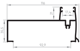
EXL-513 Complemento lateral persiana 1,015 Kg/m
