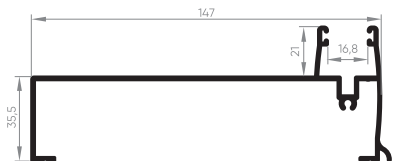
EXL-337 Complemento lateral persiana 3 planos 1,163 Kg/m
