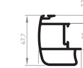
EXL-350 Montante bi-tubular central externo 0,714 Kg/m
